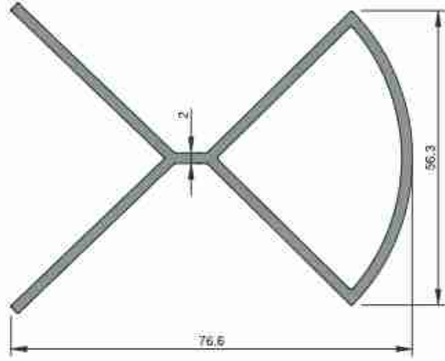
1798 1,215 kg/m
